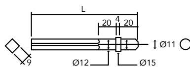
11 MM FCH-20-1F
